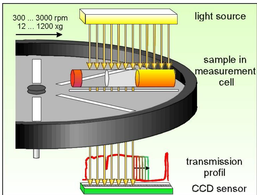
Figure 2.12. Principle of LUMiSizer dispersion analyzer. Figure adapted from Gross-Rother et al. (2018)
