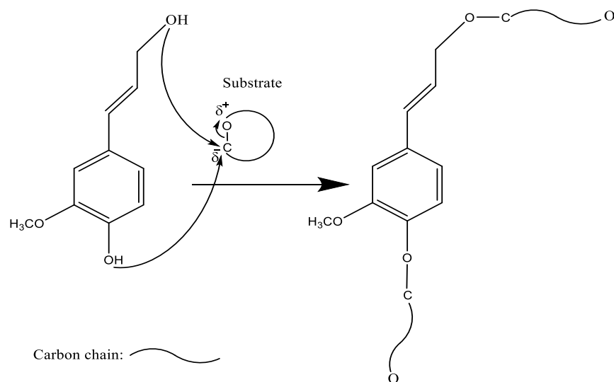
Fig. 2.5. General S_N2 reaction with ring-opening. Electrophilic center (carbon) is partially negatively-charged, and oxygen is partially positively-charged. 109,111,112
