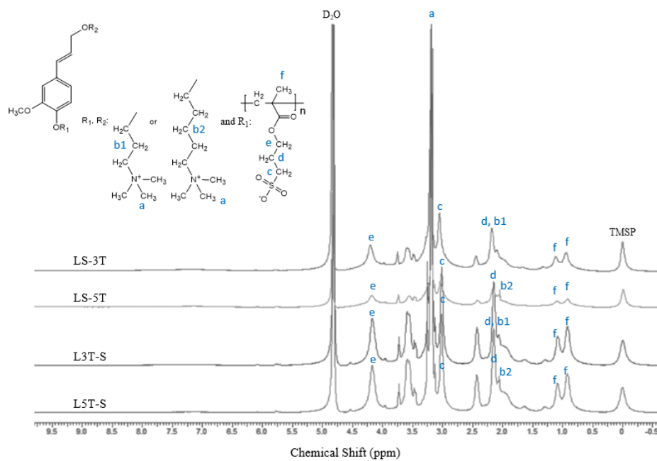
Fig. 4.3. 1 H NMR spectra of L, L-S, L-5T, and L-3T in D 2 O at 25 °C.
