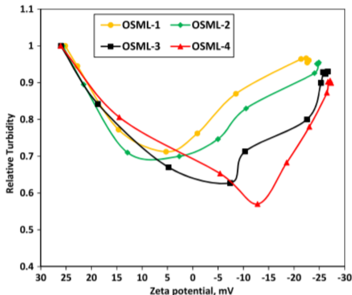
Fig. 6.4. Relationship between the relative turbidity and zeta potential of aluminum oxide suspension (25 g/L aluminum oxide suspension, pH 6)
